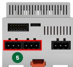
18 Wechsler-Relais-Anschlüsse
